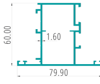
PARALLEL WINDOW OUTWARD SHUTTER PART CODE:27104
