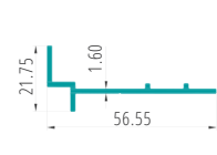
CLIP FOR LOW HEIGHT THRESHOLD PART CODE:27062
