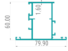
WINDOW O/W SHUTTER PART CODE:27052
