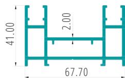
TWO TRACK PART CODE:27046
