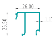
LAMINATED BEADING PART CODE:27078
