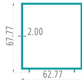
BAY POLE PART CODE:27054
