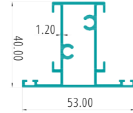
MULLION PART CODE:27084
