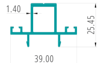
CENTRE LOCKING H PLATE PART CODE:27031
