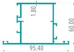
DOOR O/W SHUTTER PART CODE:27048
