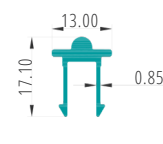
GUIDE RAIL PART CODE:27021
