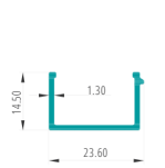
LAMINATED REDUCER FOR SLIM SHUTTER PART CODE:27091
