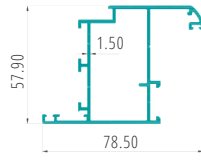
WINDOW I/W SHUTTER PART CODE:27065
