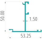
INVERSION PART CODE:27080
