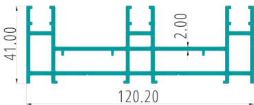
THREE TRACK PART CODE:27025
