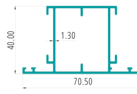
DOOR O/W SHUTTER PART CODE:62190
