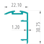
MESH SHUTTER INTERLOCK PART CODE:62484
