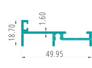
LOW HEIGHT THRESHOLD PART CODE:27063
