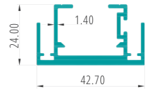
SLIM SGU DOUBLE INTERLOCK PART CODE:27092
