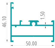
WINDOW FRAME PART CODE:62387
