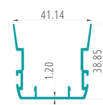
DOUBLE INTERLOCK PART CODE:27068
