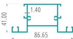
MESH SHUTTER MULLION PART CODE:27045
