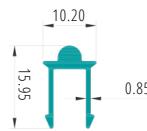
GUIDE RAIL PART CODE:27073
