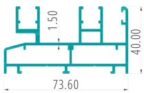
TWO TRACK PART CODE:27013
