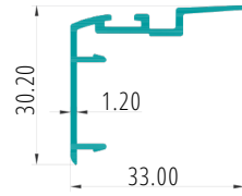
INTERLOCK PART CODE:27072
