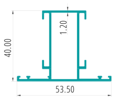
MULLION PART CODE:62132
