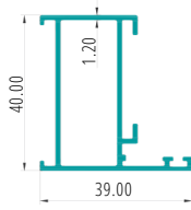
WINDOW FRAME PART CODE:62133
