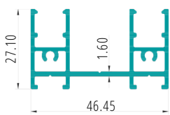
TWO TRACK PART CODE:27069
