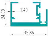
SLIM SGU INTERLOCK PART CODE:27019
