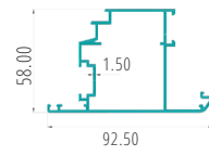
DOOR O/W SHUTTER PART CODE:62392
