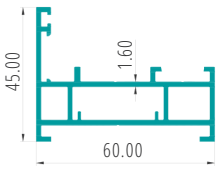
PARALLEL WINDOW FRAME PART CODE:27103
