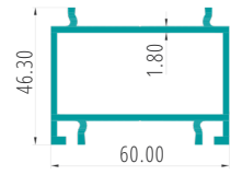
EXTENSION FRAME PART CODE:27051
