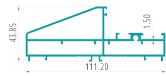
THREE TRACK FIX FRAME PART CODE:27012
