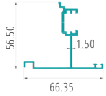
DUMMY MULLION PART CODE:27081
