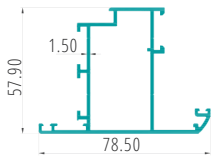
WINDOW O/W SHUTTER PART CODE:62389
