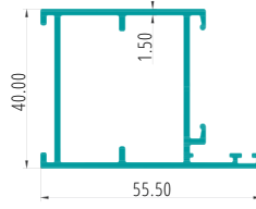
DOOR FRAME PART CODE:62334
