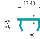
MESH BEADING PART CODE:27074
