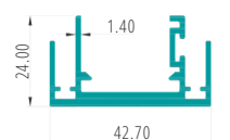
SLIM DGU DOUBLE INTERLOCK PART CODE:27090
