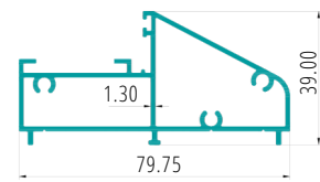
THREE TRACK FIX FRAME PART CODE:27094
