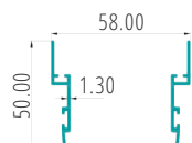
DOUBLE INTERLOCK PART CODE:27030
