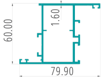
WINDOW I/W SHUTTER PART CODE:27053
