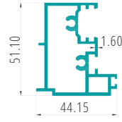
DUMMY MULLION PART CODE:27050
