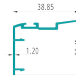
INTERLOCK PART CODE:62463
