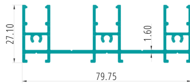
THREE TRACK PART CODE:27070
