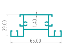
MESH SHUTTER MULLION PART CODE:27042
