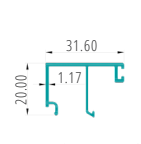
MESH BEADING PART CODE:27028
