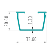
SGU REDUCER PART CODE:27032
