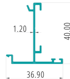
INVERSION PART CODE:27083
