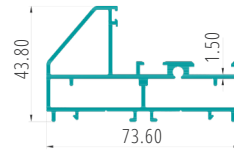
TWO TRACK FIX FRAME PART CODE:27014
