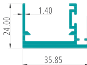
SLIM DGU INTERLOCK PART CODE:27089
