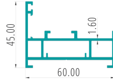
TOP HUNG FRAME PART CODE:27057
