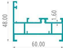
WINDOW FRAME PART CODE:27055
