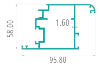
DOOR I/W SHUTTER PART CODE:62391
