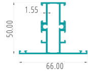
MULLION PART CODE:62388
