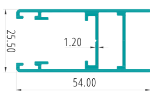
SHUTTER PART CODE:27071
