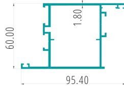
DOOR I/W SHUTTER PART CODE:27049
