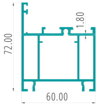
DOOR FRAME PART CODE:27047
