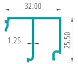
SGU BEADING PART CODE:62394
