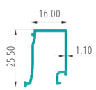
DGU BEADING PART CODE:62375
