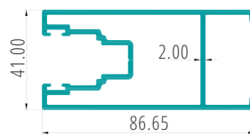
GLASS SHUTTER PART CODE:27026
