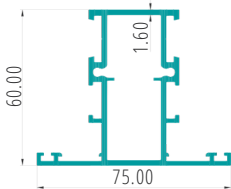
MULLION PART CODE:27056
