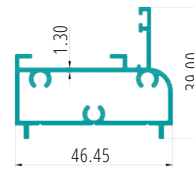
TWO TRACK FIX FRAME PART CODE:27095
