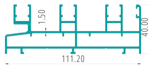
THREE TRACK PART CODE:27011
