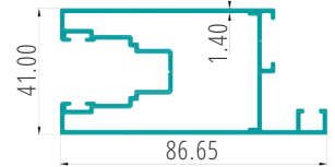
MESH SHUTTER PART CODE:27027
